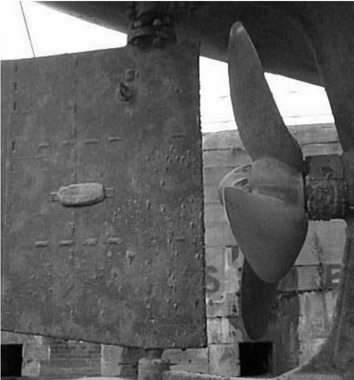
Figure 4 The rudder and propeller of a small vessel in dry dock
